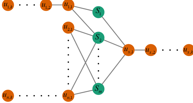
Fig. S2. The static bump hunting problem is NP-hard when \alpha = 1 .
