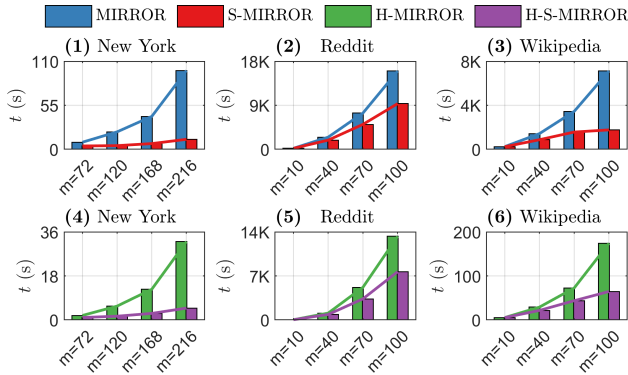
Figure 4: Nearly quadratic and linear scalabilities to m .
