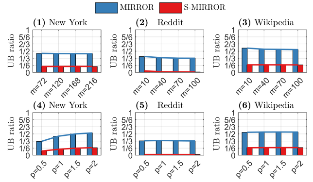
Figure 5: Upper bound ratios of MIRROR and S-MIRROR.
