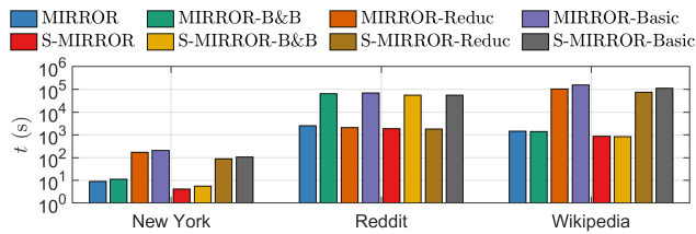
Figure 6: The effectiveness of acceleration techniques.
