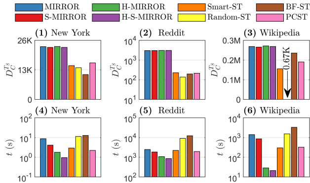
Figure 2: Comparison of solution quality and speed.
